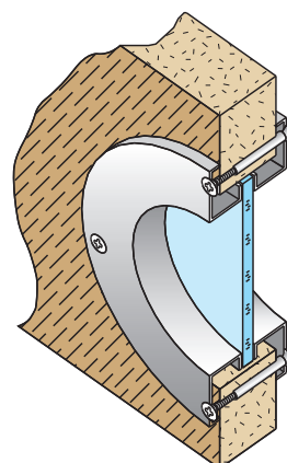
FP (Thru-Bolted)
